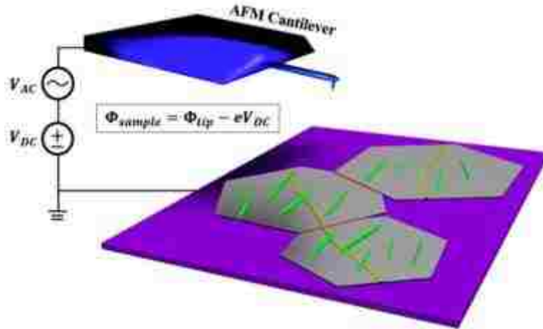
Figure 2–11 Schematic of Kelvin probe force microscopy 63
