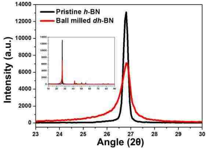
Figure 3–3 Zoomed in XRD spectra of pristine h -BN (black) and ball milled dh -BN (red) powders. The inset provides the XRD spectra with the 2\theta ranging from 10 to 90^\circ .
