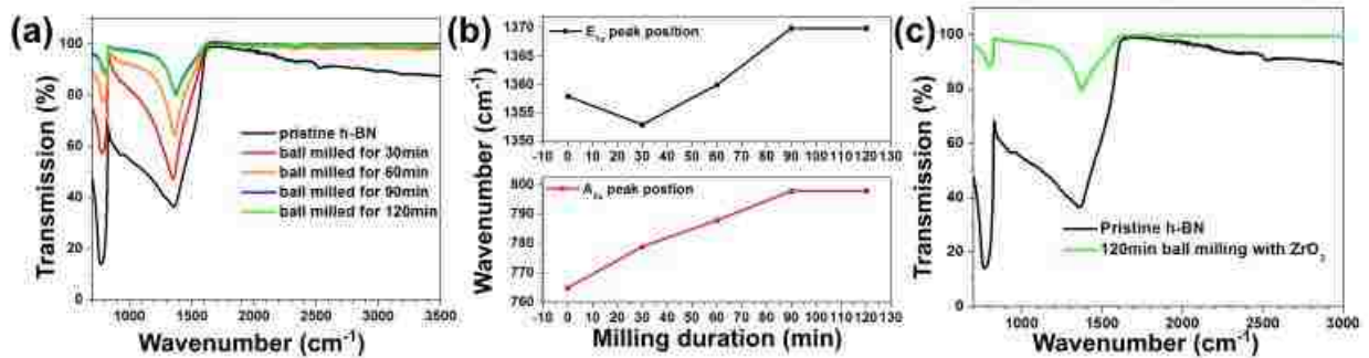
Figure 3–5 (a) FTIR spectra of h -BN and dh -BN obtained for milling times of 30 min, 60 min, 90 min, and 120 min with ZrO_2 . (b) Evolution of E_{1u} (top, black) and A_{2u} (bottom, red) IR bands as a function of milling duration. (c) FTIR spectra of h -BN and dh -BN obtained after ball milling for 120 min with ZrO_2 (green) milling balls.
