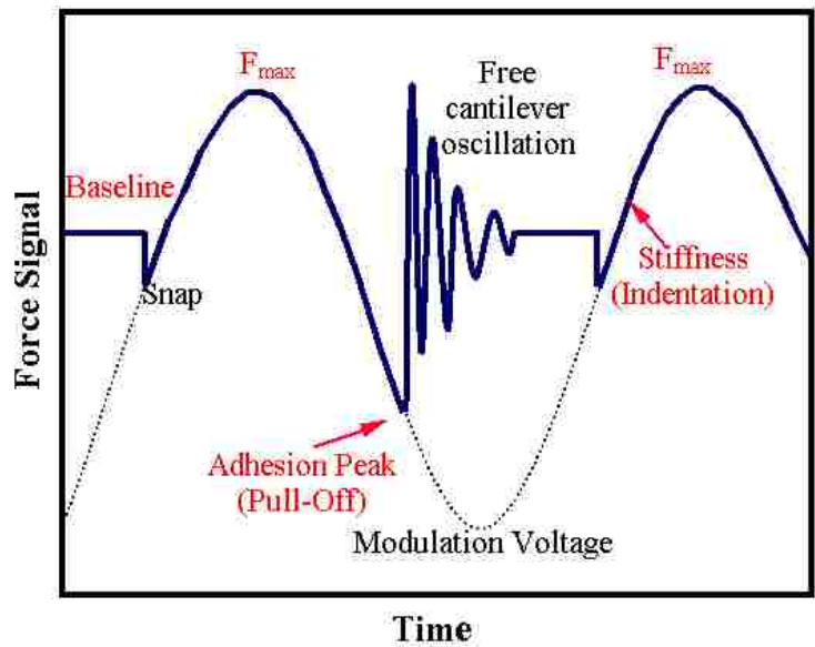
Figure A-2 Representative PFM curve (purple bold line) with sinusoidal modulation (dotted line), attributes related to stiffness, adhesion peak and F_{max} indicated on the curve
