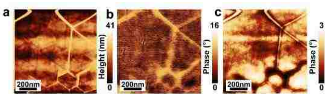
Figure 4–5 Nanoscale functional imaging to of heated-treated h -BN (a) AFM morphology and corresponding (b) EFM phase image with +3V tip bias, (c) EFM phase image with -3V tip bias
