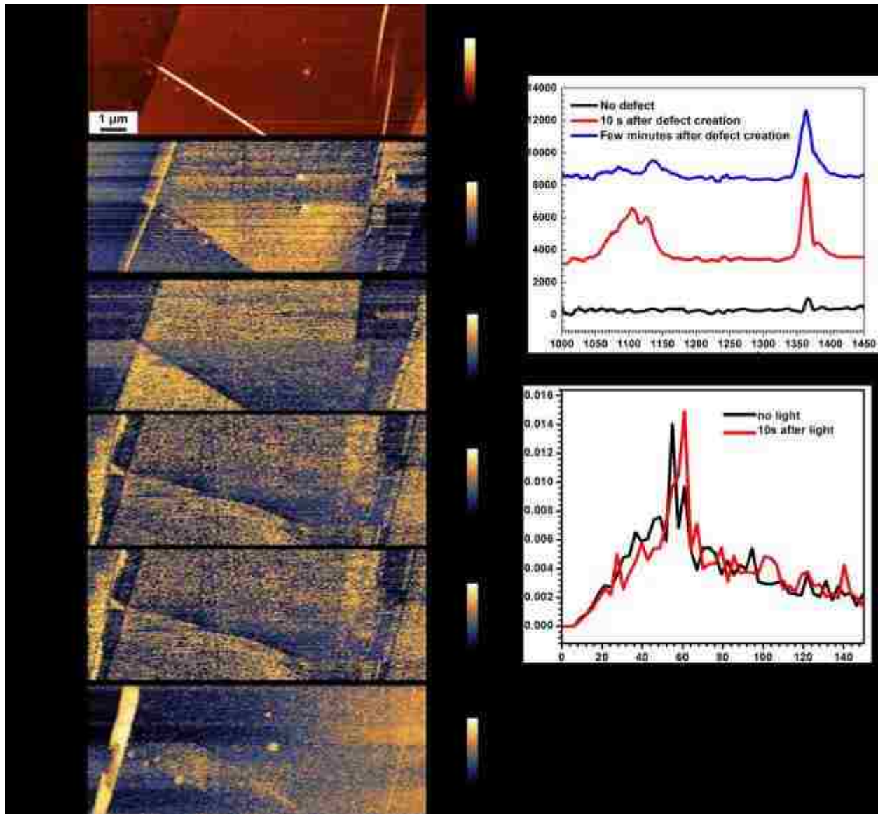
Figure 4–12 Reactions over laser induced defect sites. (a) AFM topography image of BN flake with laser induced defect sites; (b-f) NanoIR amplitude maps obtained at different wavenumbers; (g) NanoIR spectra acquired from the same position at two different time points; (h) Contact resonant frequency of the AFM cantilever showing the frequency shift
